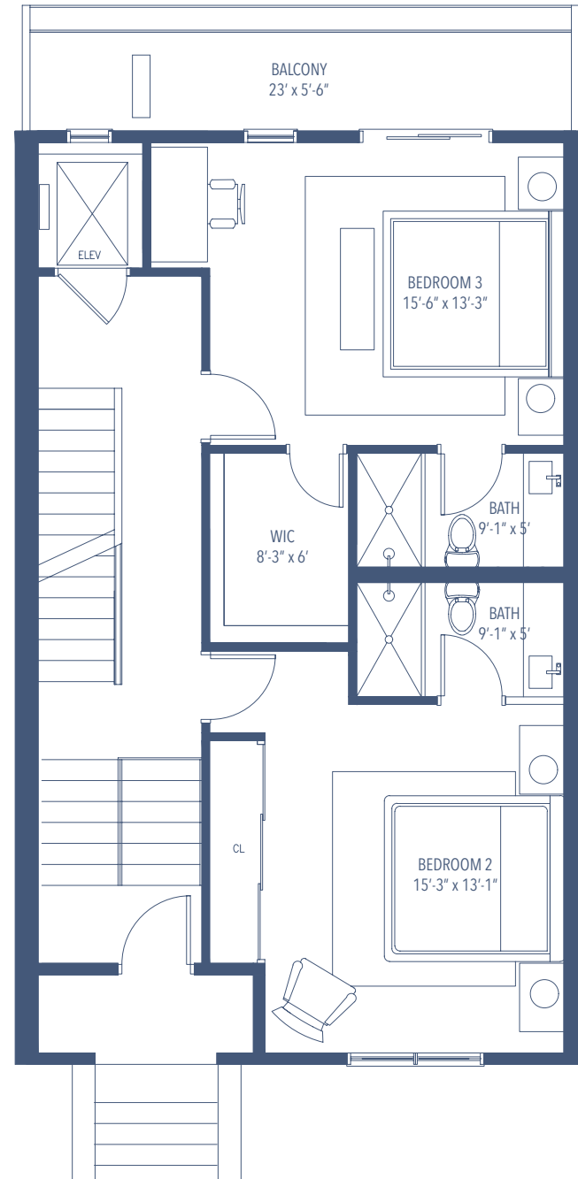
FIRST LEVEL
